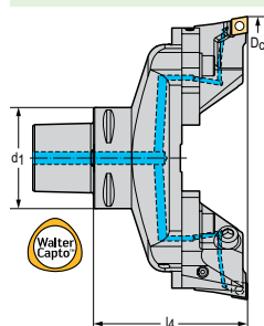
Walter Capto™ in acc. with ISO 26623
