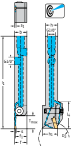
Square shank
